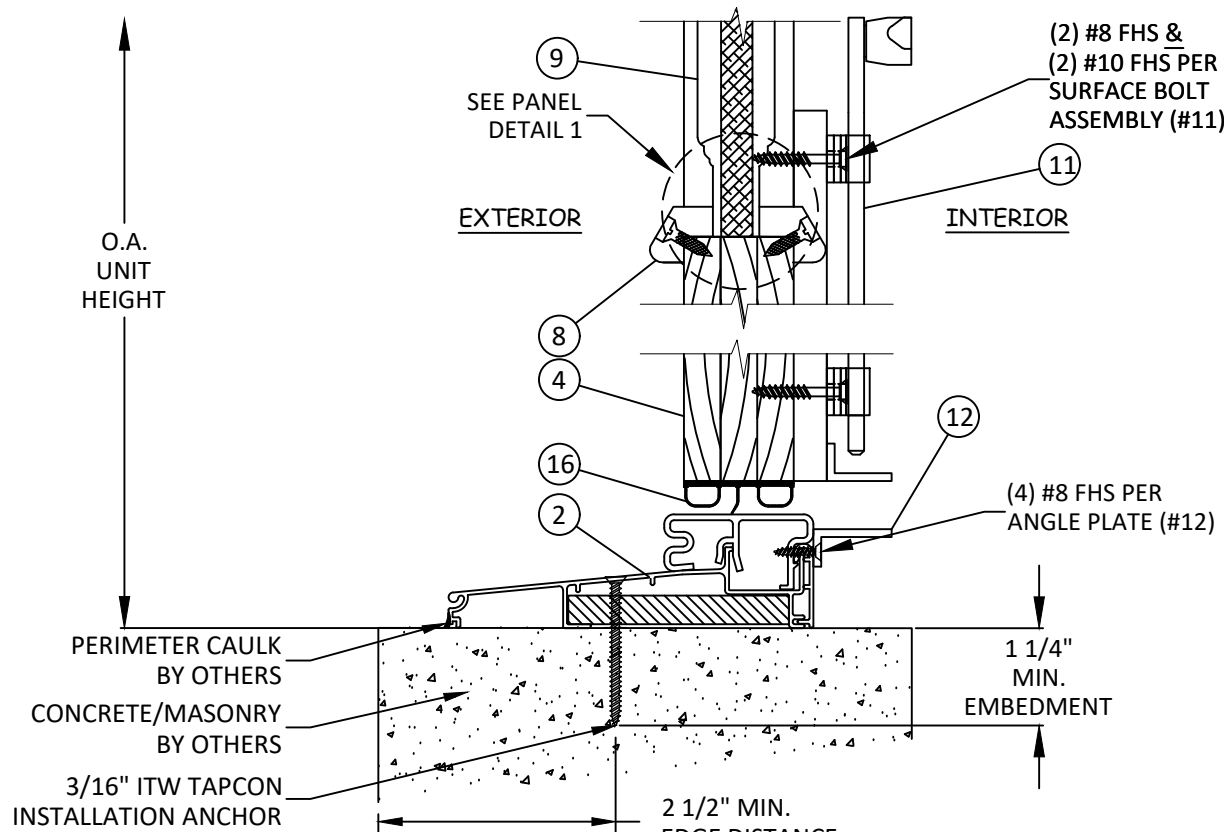
A 4 VERTICAL SECTION SILL - CONCRETE/MASONRY
