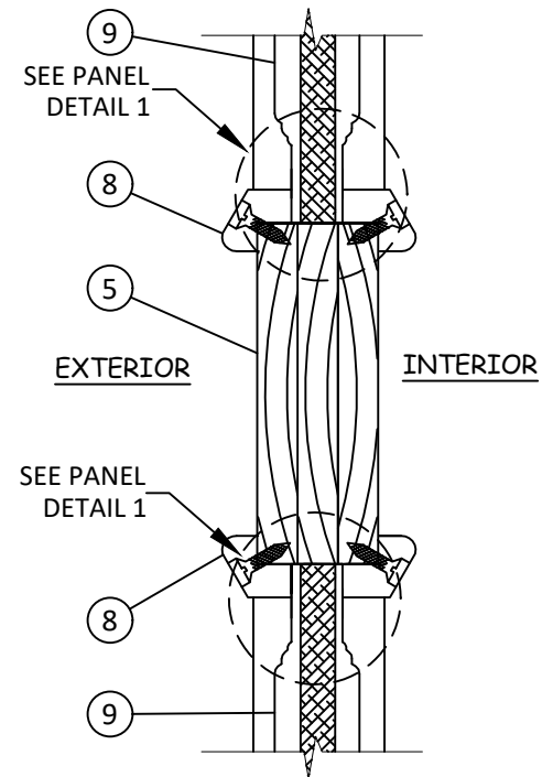
D 4 VERTICAL SECTION MIDRAIL - OPAQUE
