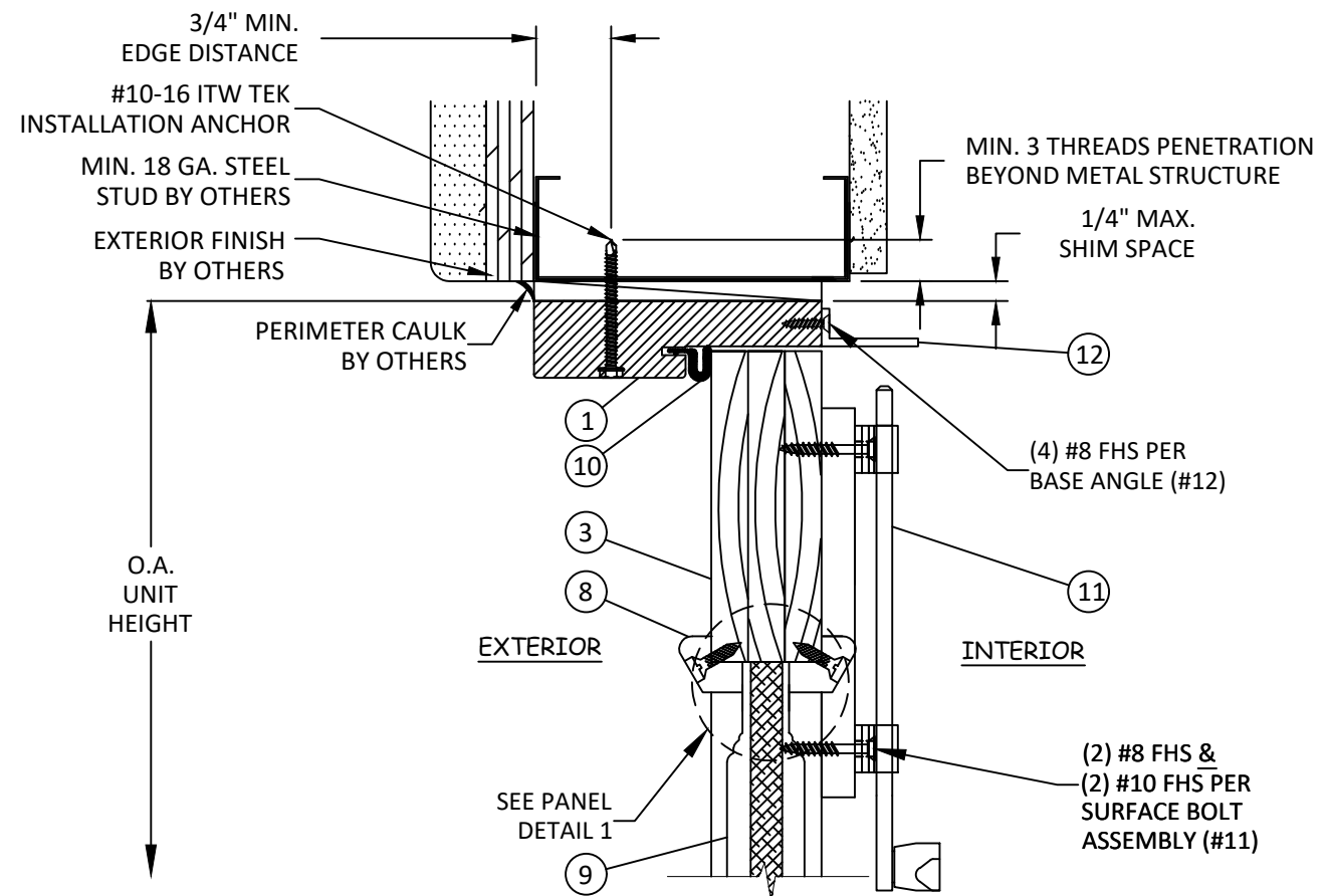
C 4 VERTICAL SECTION HEAD - STEEL STUD
