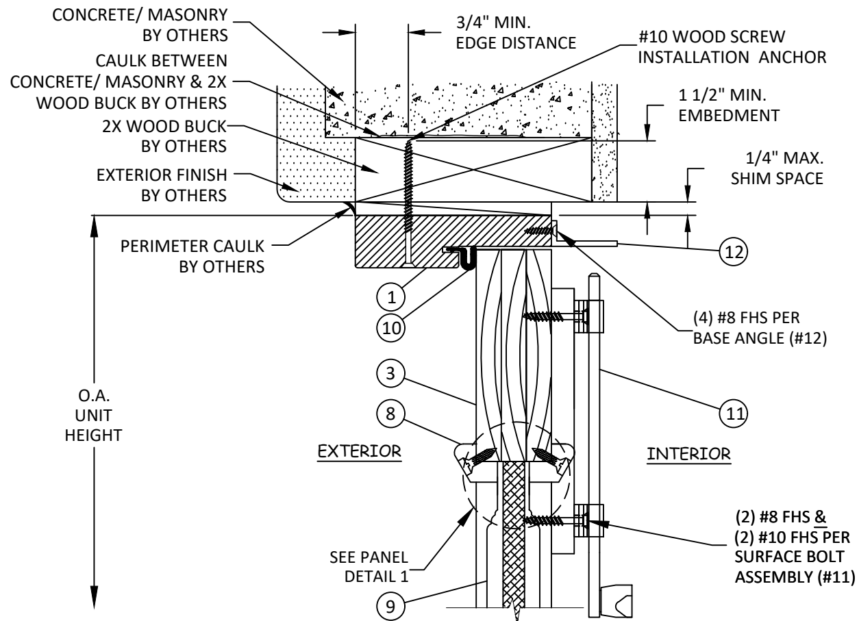
B 4 VERTICAL SECTION HEAD - 2X WOOD BUCK
