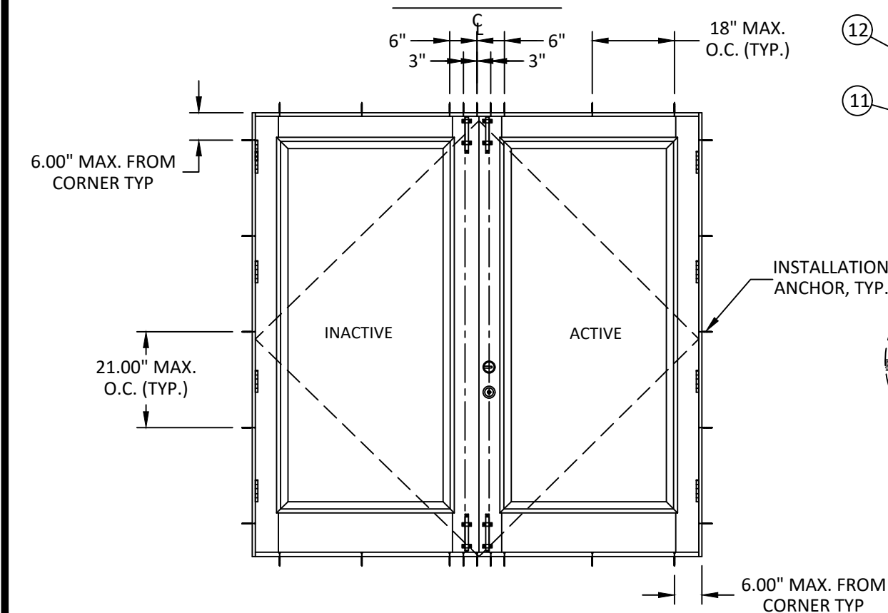
ANCHOR LAYOUT
